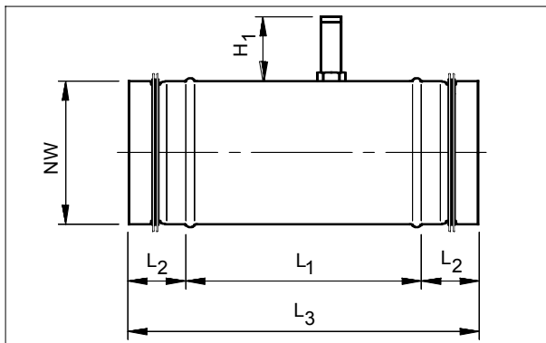
Version without insulating shell
